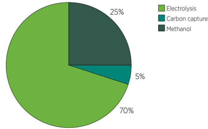
Figure 3. Estimated distribution of heat production from a PtX chain of electrolysis, carbon capture and methanol production. It is assumed that all of the hydrogen and CO 2 is converted into methanol. Parts of the heat from the methanol and electrolysis process will require a heat pump. The figures do not include heat integration and optimisation in the PtX chain.
