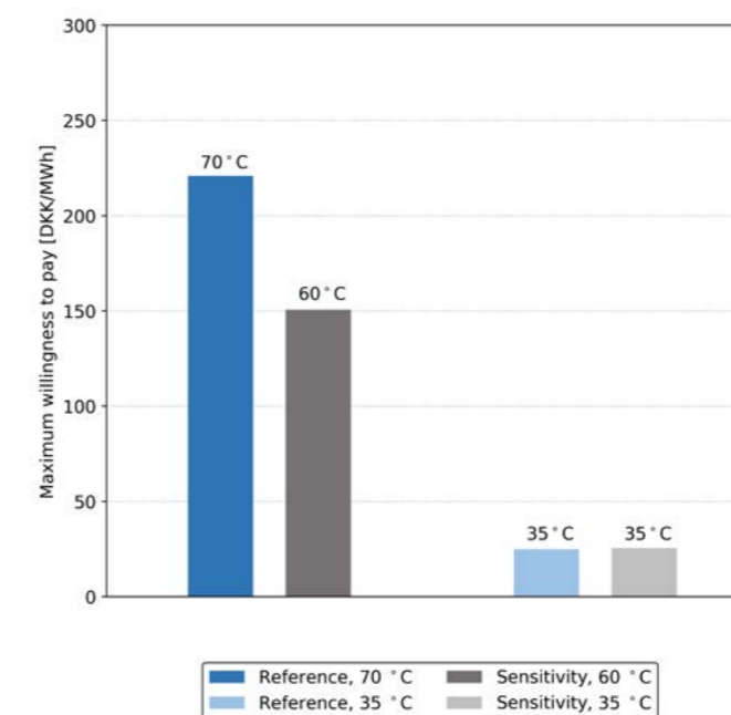
Figure C4: Maximum willingness to pay for 70 °C waste heat and for 60 °C waste heat on an annual basis for Scenario 3, and the maximum willingness to pay for 35 °C waste heat. The willingness to pay is lower for 60 °C waste heat because the other units need to provide additional heat output hereby increasing the overall costs.
