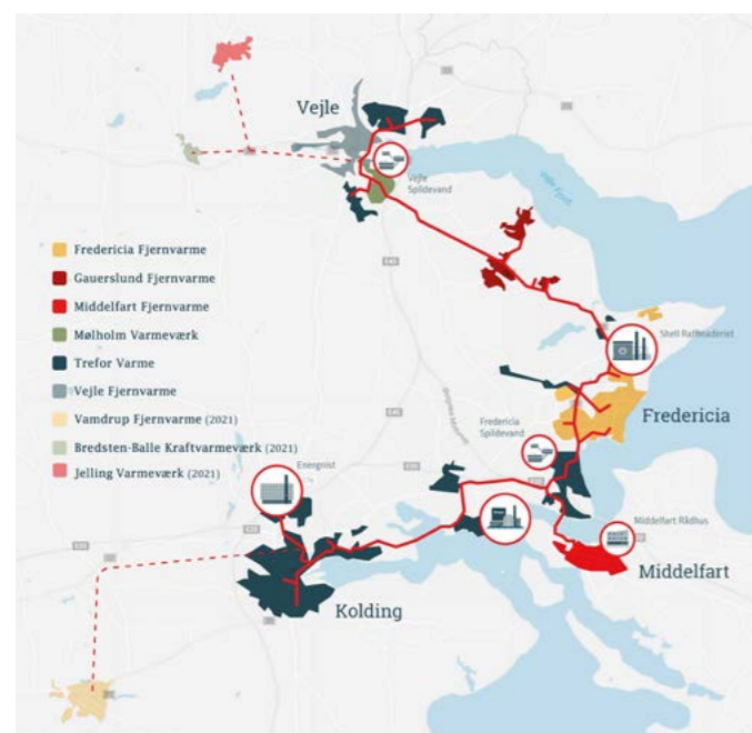
Figure 19. Heat transmission in the Triangle Region combines heat production and local district heating areas via the TVIS district heating transmission grid (red lines). Source: TVIS.net
