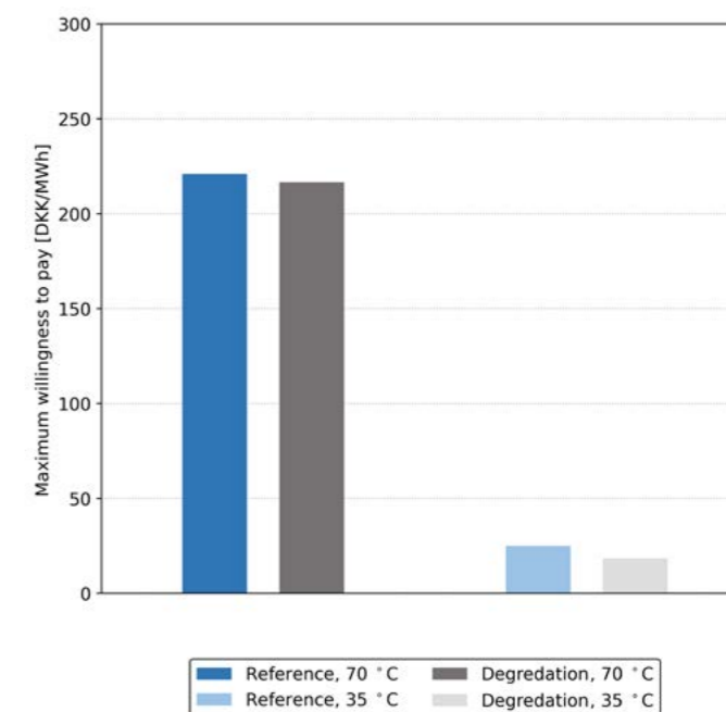
Figure C5: Maximum willingness to pay for 70 °C waste heat and 70 °C waste heat with a degraded stack in Scenario 3. The willingness to pay is lower with the degraded stack because the electrolysis plant has fewer operating hours and therefore does not replace as much costly heat production.
